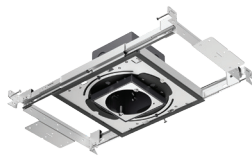
M4NCSS New Construction Standard
